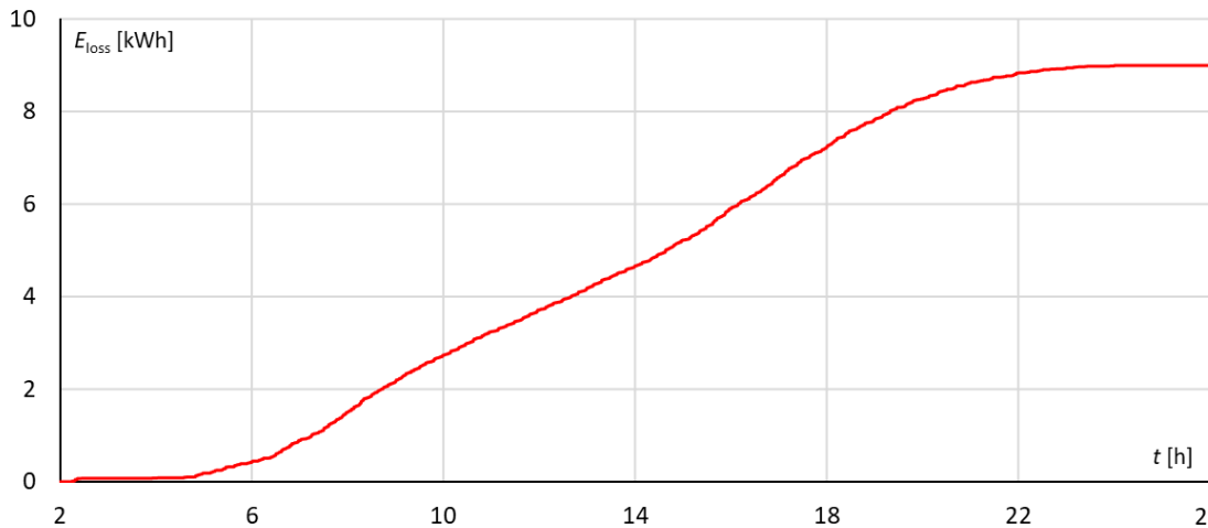
Fig. 6.38. Feeder losses energy – substation Gdynia Redłowo
