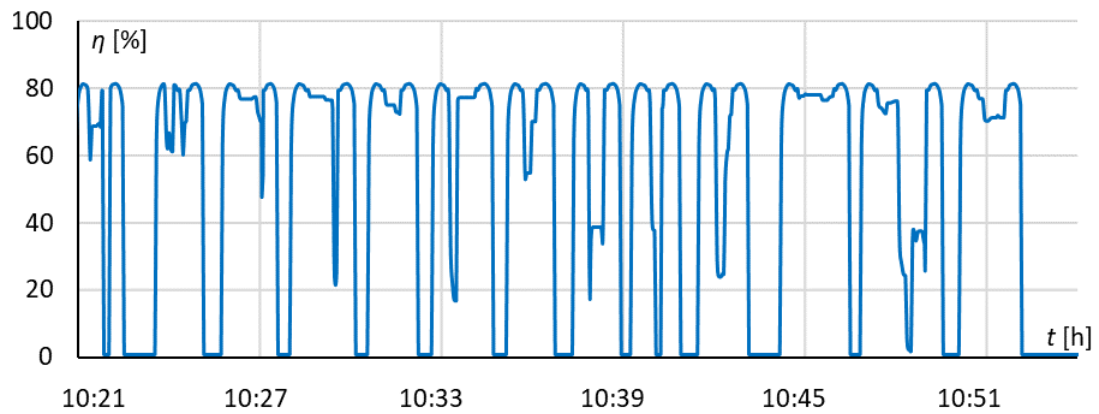
EN71SKM – drivetrain efficiency waveform, track 501
