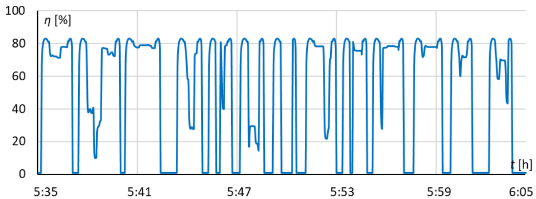
31WE – drivetrain efficiency waveform, track 502
