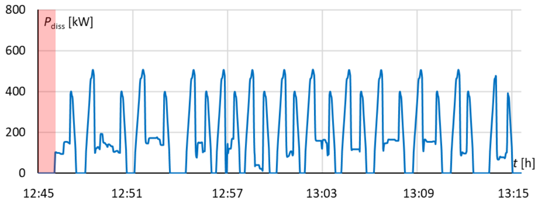
Fig. 6.8. Simulated traction drive losses power – EN57AKM, track 502
