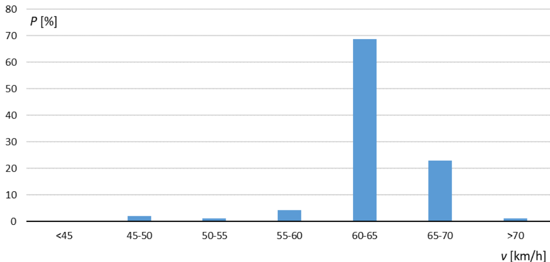
Fig. 5.38. Percentage of cruising velocities – track 502 (direction Gdańsk)
