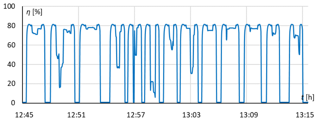
Fig. 6.7. Simulated traction drive efficiency – EN57AKM, track 502
