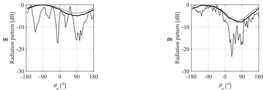
Fig. 2. Radiation patterns in yz-plane (cf. Fig. 1) obtained from AC (gray) and the non-anechoic measurements (black) before (···), and after correction (—) at: (a) 4 GHz and (b) 7 GHz frequencies.
